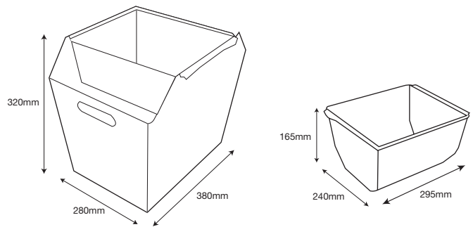
nominal dimensions
