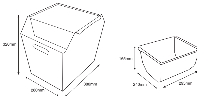
nominal dimensions
